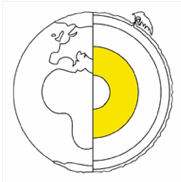
outer core
