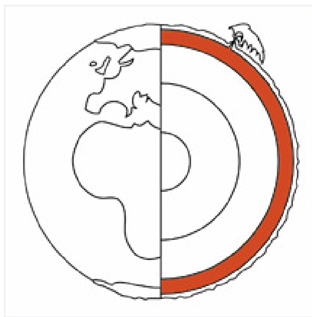
upper mantle
