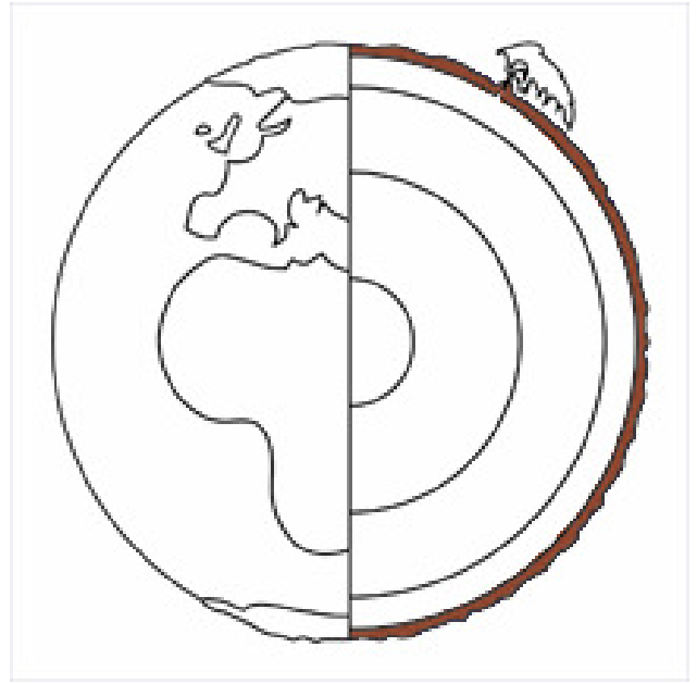
crust
